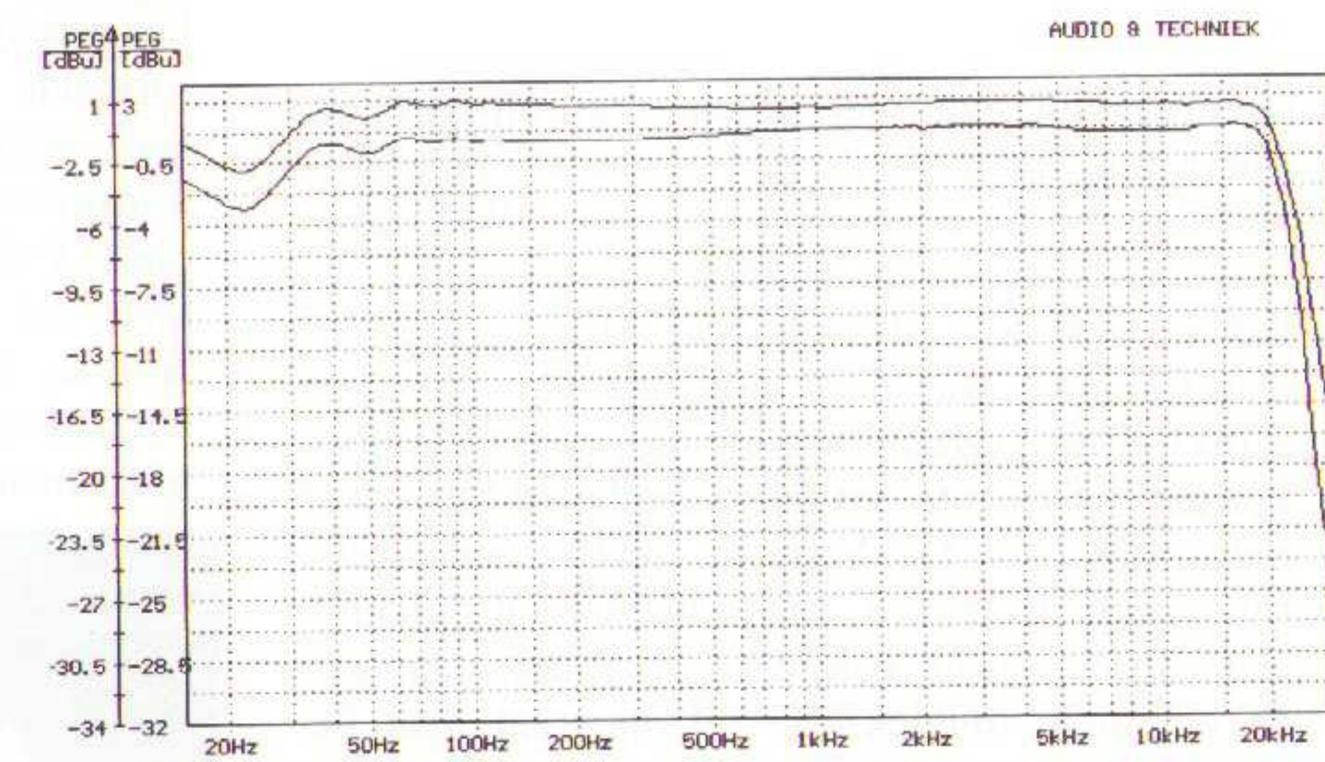
Yamaha KX-650
